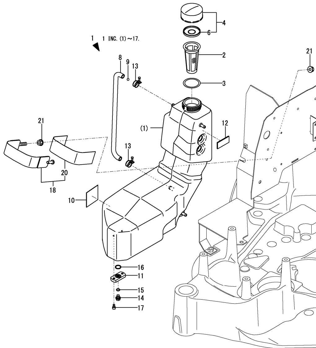
Fig.7. FUEL TANK
