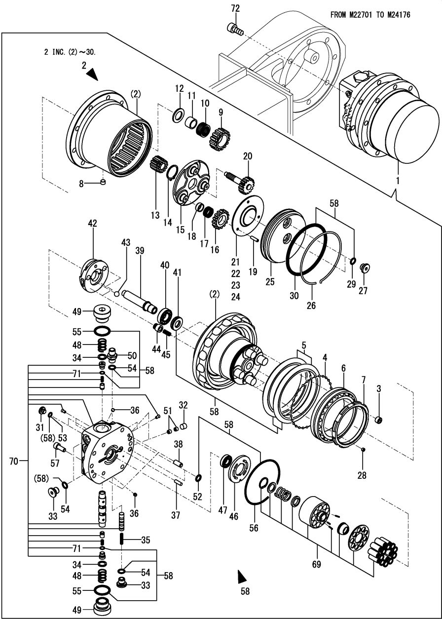
Fig.33. TRAVEL MOTOR(K)
