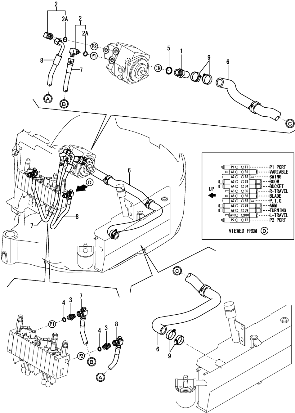
Fig.45. TANK - PUMP - VALVE(PUMP : K SPEC.)(TO M28674)
