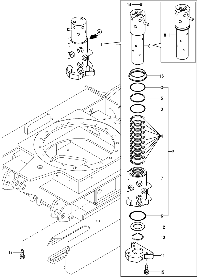
Fig.35. SWIVEL JOINT(Y SPEC.)(TO M28357)
