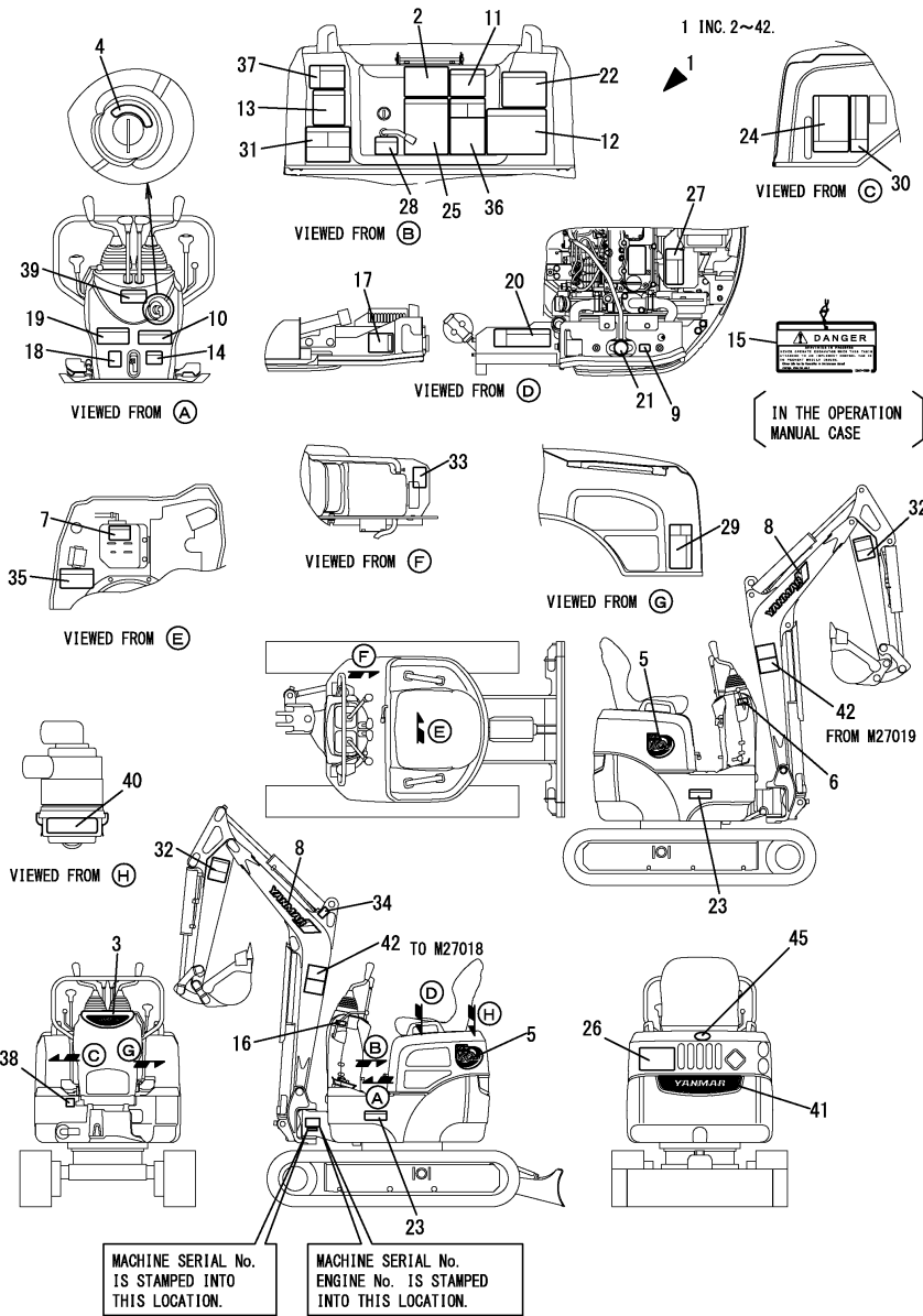
Fig.1. LABEL(VIO10-2A)(TO M2F000)
