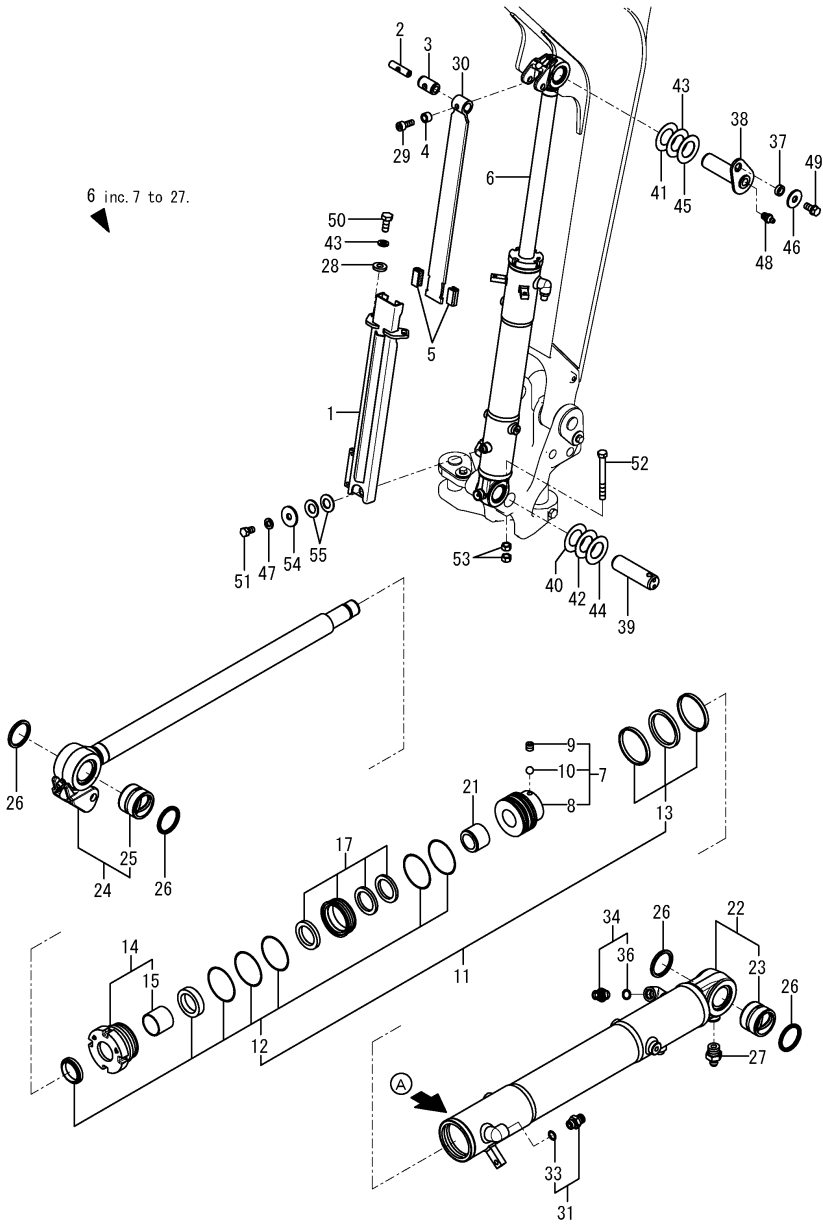
Fig.82. BOOM CYLINDER(TO M66175)
