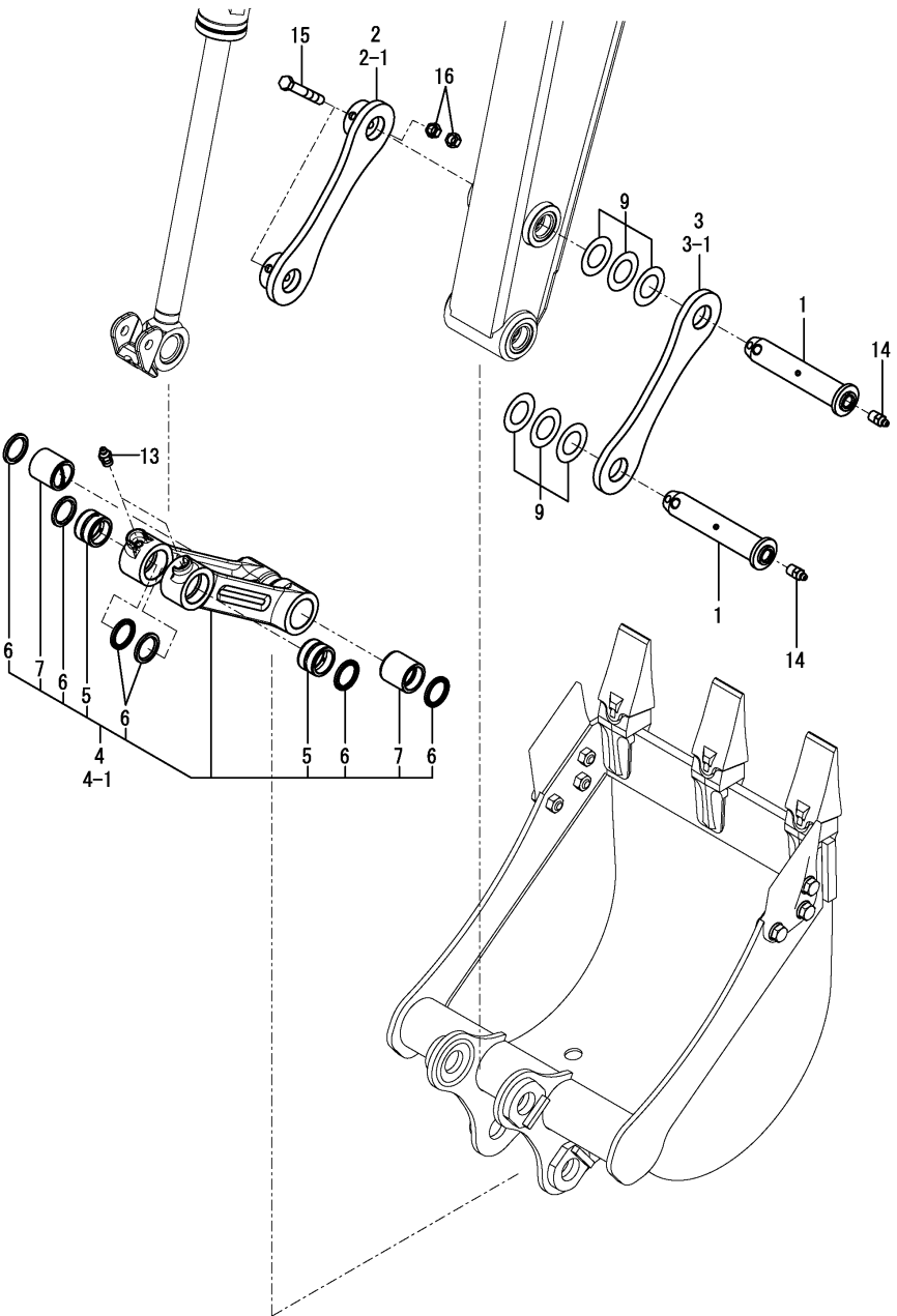
OCK50-M02280 IMPLEMENT Fig.123. BUCKET ARM & LINK
