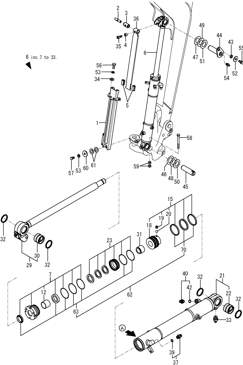
Fig.131. (82A)BOOM CYLINDER(FROM M66176)
