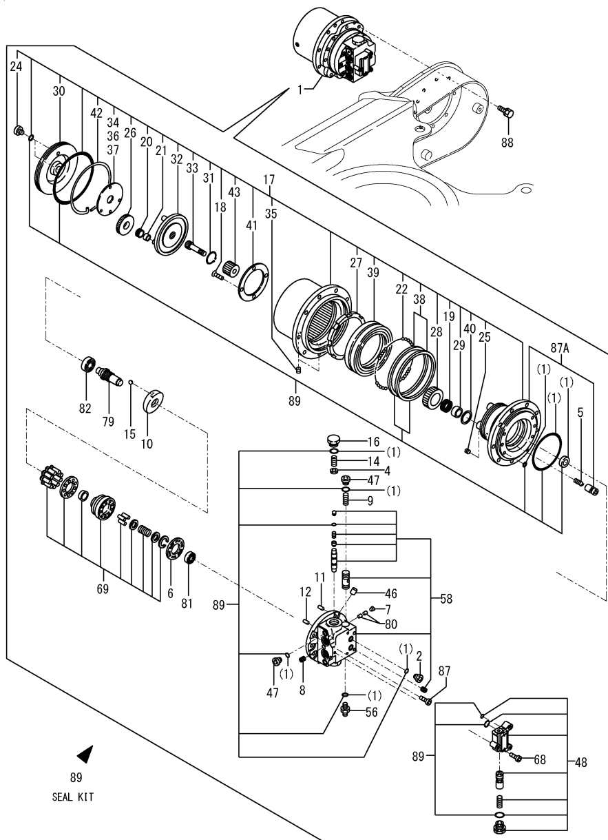
Fig.88. TRAVEL MOTOR
