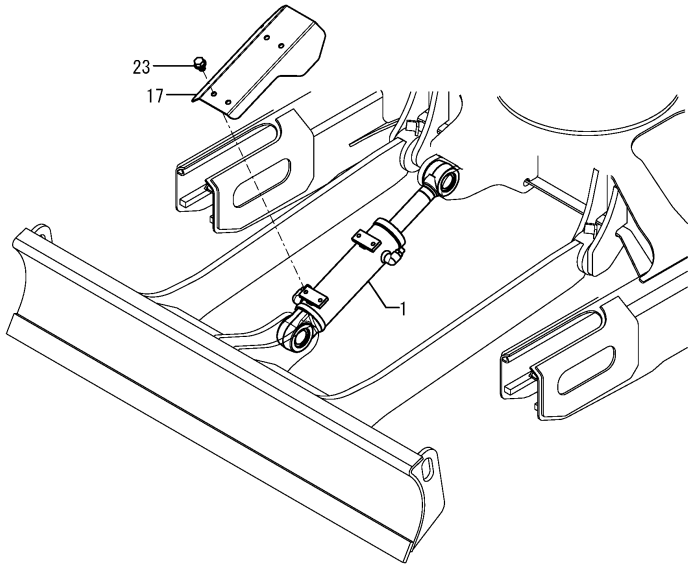
Fig.86. BLADE CYLINDER(TO M66162)
