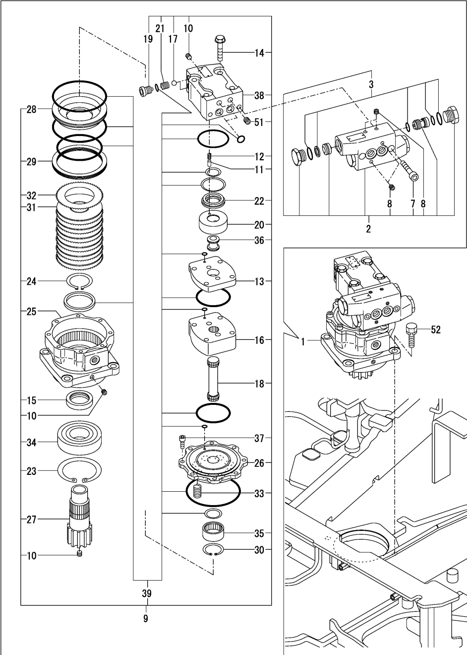
Fig.89. TURNING MOTOR
