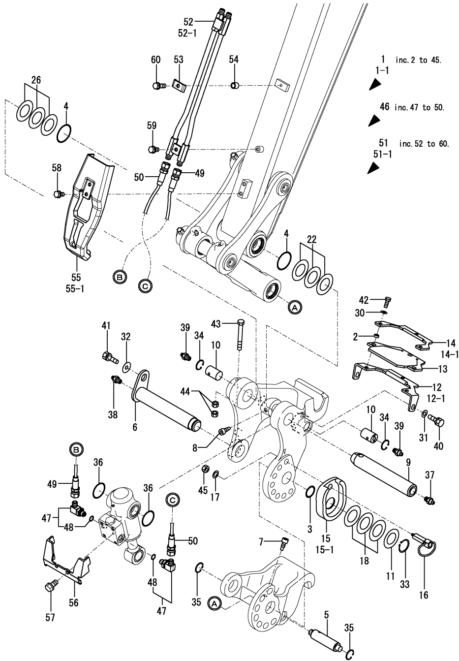
Fig.129. OVERHAUL KIT(QUICK COUPLER)(OPTIONAL)
