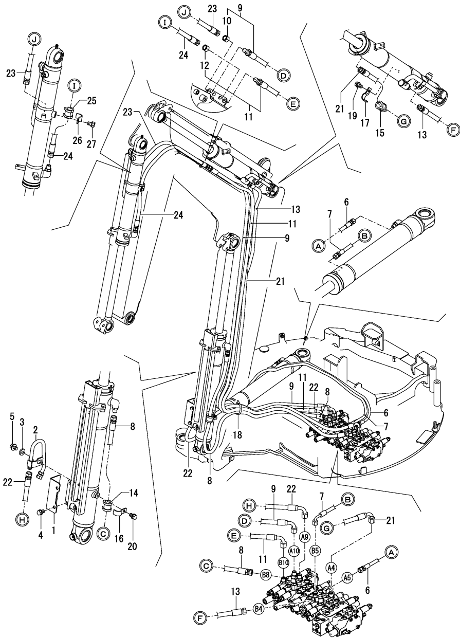
Fig.109. CONTROL VALVE - IMPLEMENT CYLINDER
