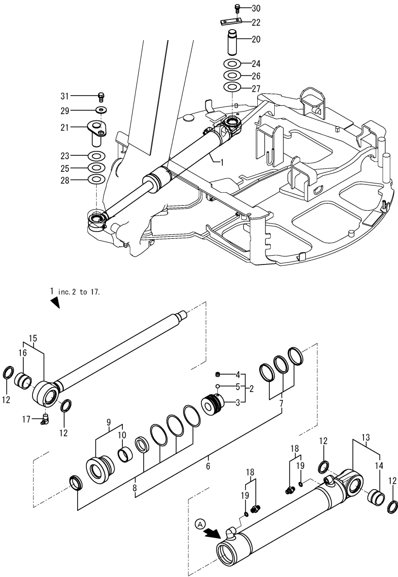
Fig.85. SWING CYLINDER(TO M66186)
