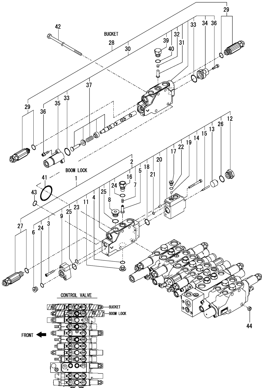
Fig.93. CONTROL VALVE(2/7)
