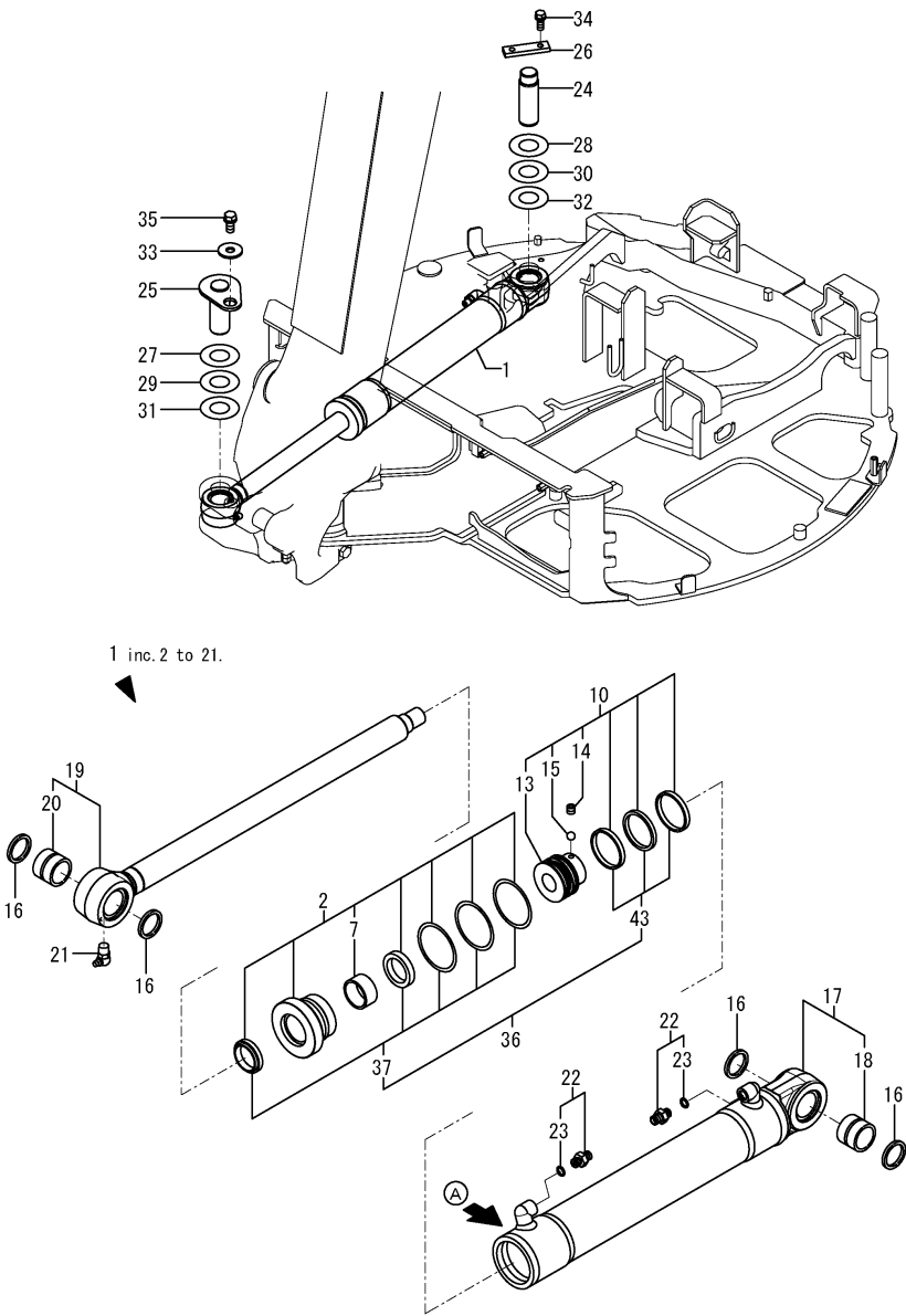
Fig.133. (85A)SWING CYLINDER(FROM M66187)
