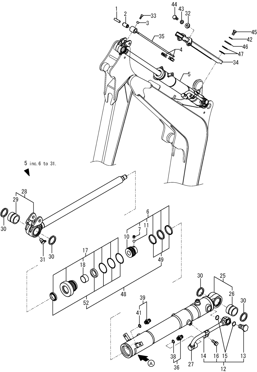
Fig.132. (83A)ARM CYLINDER(FROM M66187)
