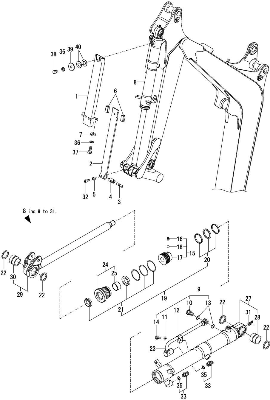
Fig.84. BUCKET CYLINDER(QUICK COUPLER SPEC.)
