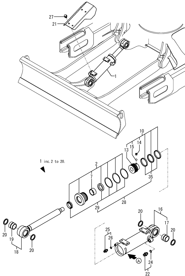
Fig.134. (86A)BLADE CYLINDER(FROM M66163)
