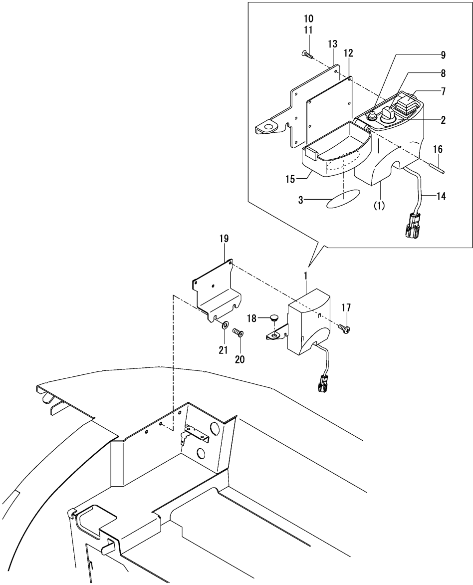
Fig.33. QUICK COUPLER(SWITCH BOX)
