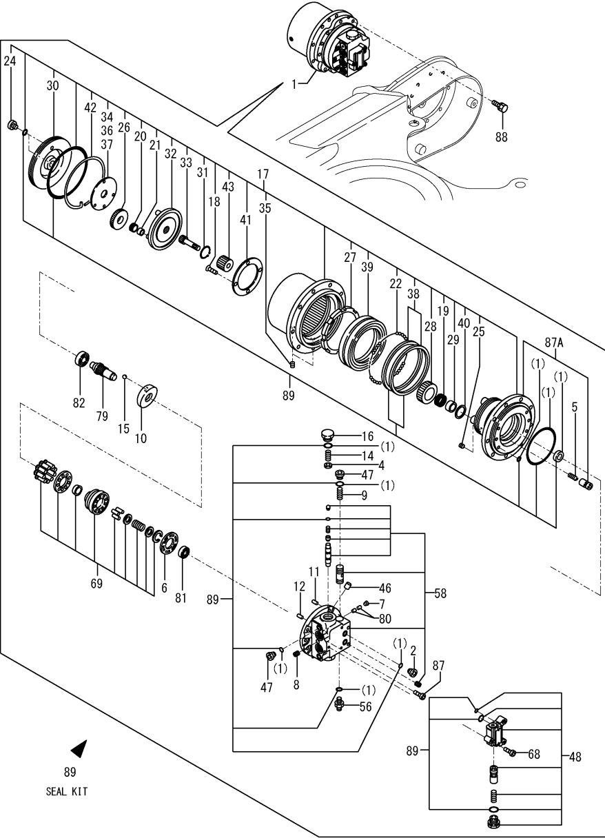
Fig.88. TRAVEL MOTOR
