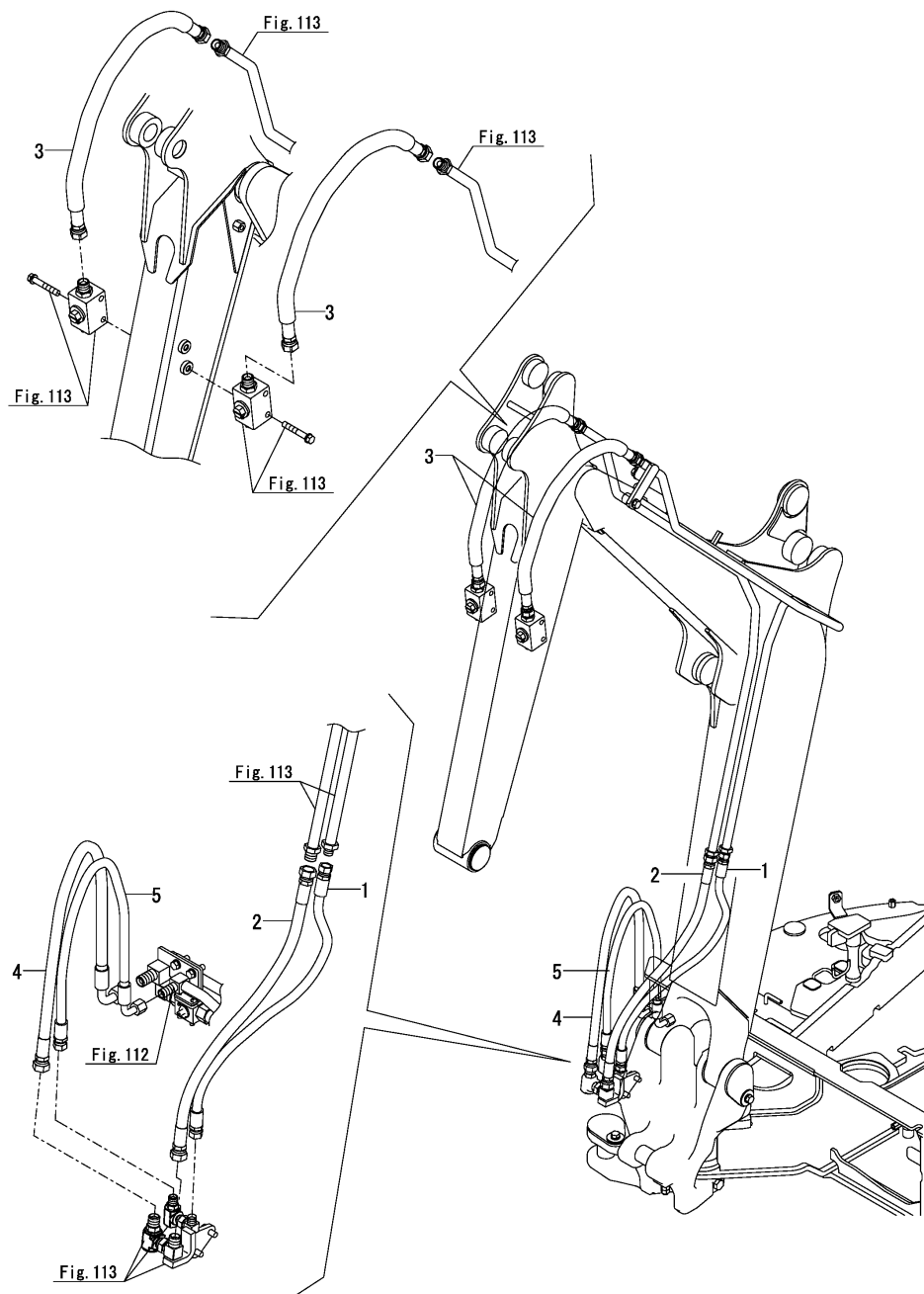
Fig.114. P.T.O.(ARM END)(2)
