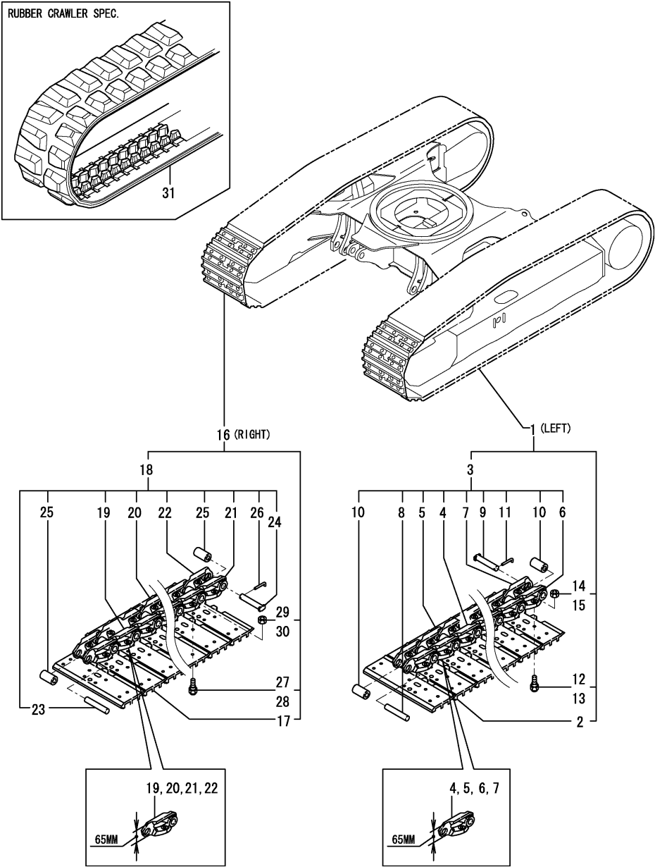
Fig.156. (22A)CRAWLER(FROM M59061)
