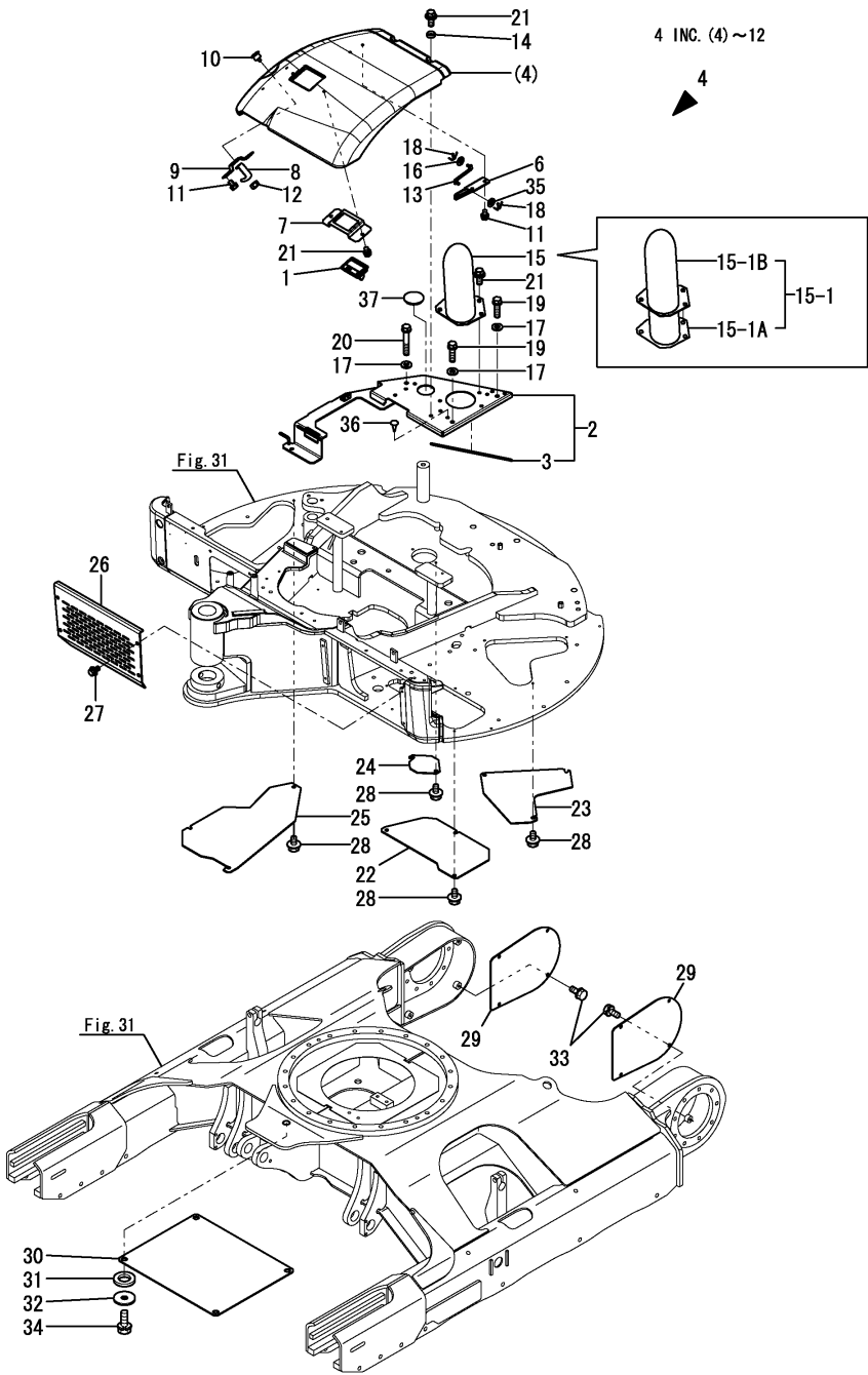
0CS10-M51901 COVER Fig.32. COVER(FRAME)
