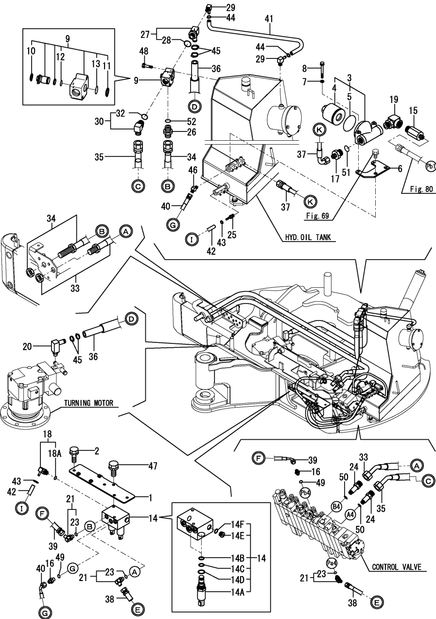
OCS10-M51901 HYDRAULIC OIL PIPING Fig.124. P.T.O.(PPC)(FRAME END)
