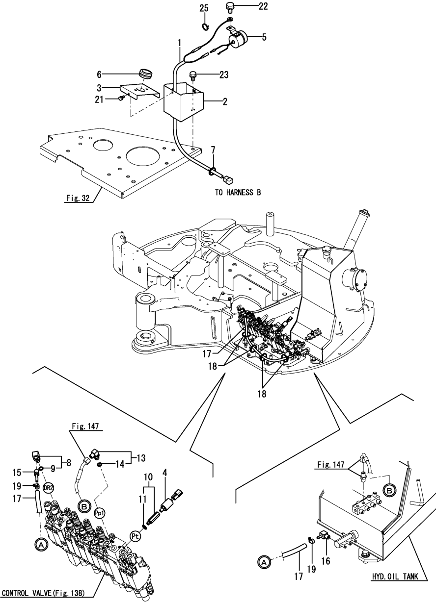
Fig.136. (13A)TRAVEL ALARM(US : FROM M54866)
