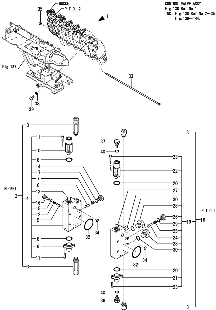
Fig.138. (59A)CONTROL VALVE(1/7)(US : FROM M54866)
