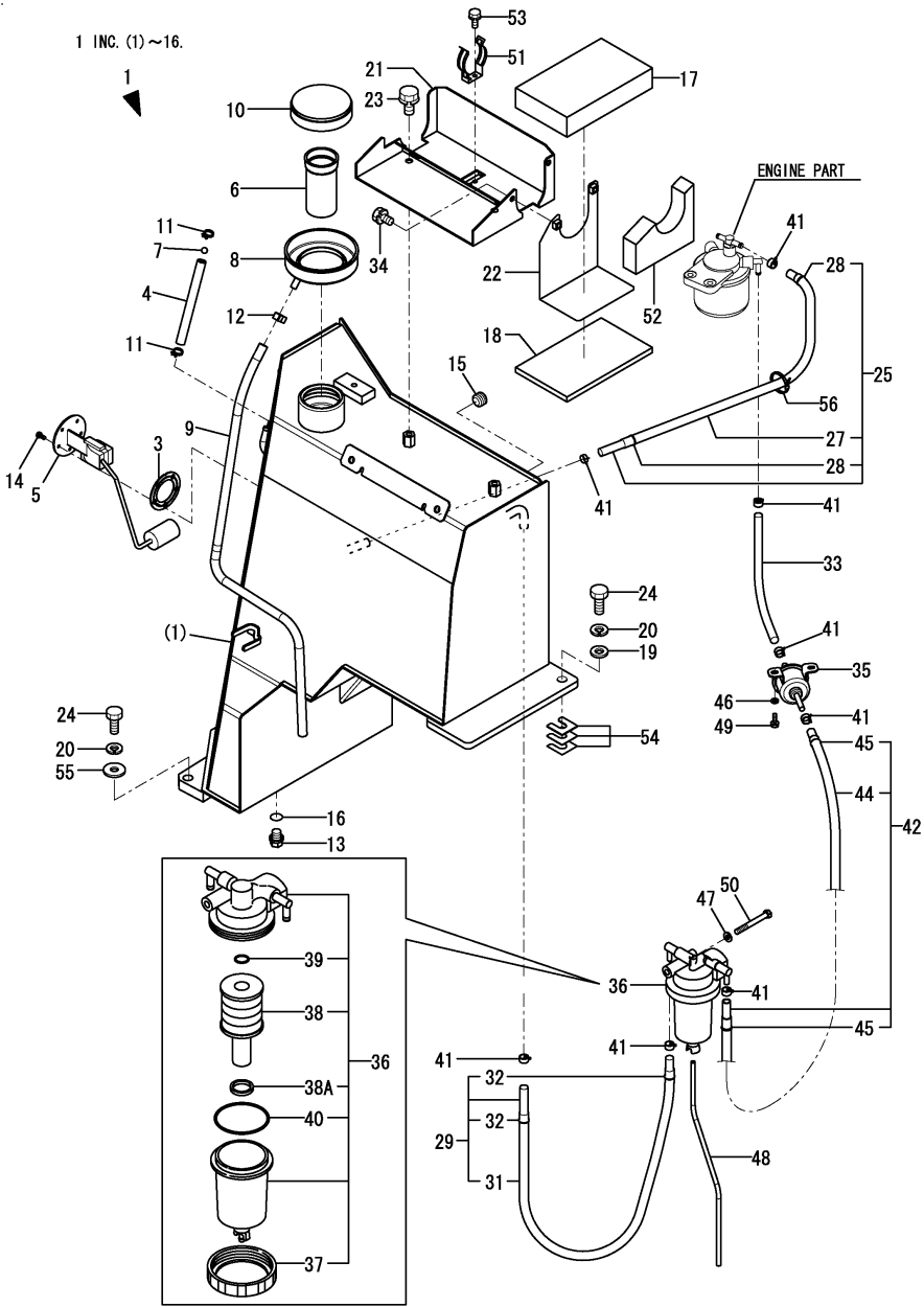
Fig.8. FUEL TANK & FUEL PIPING
