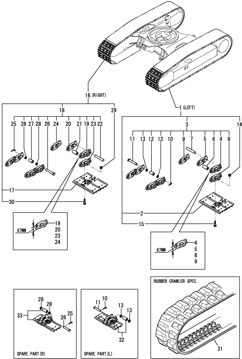
OCS10-M51901 TRAVELING Fig.22. CRAWLER(TO M59060)
