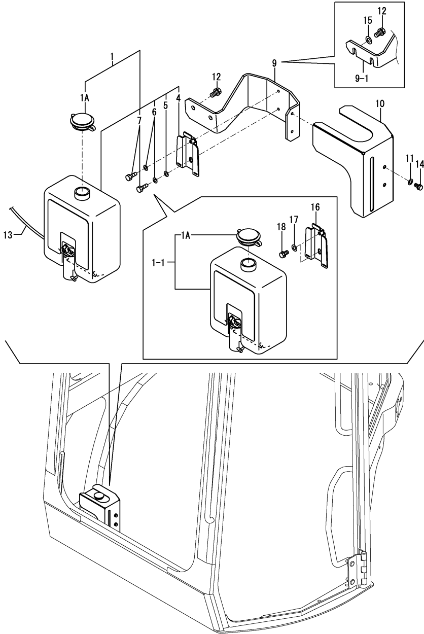
OCS10-M51901 CABIN Fig.17. WINDOW WASHER
