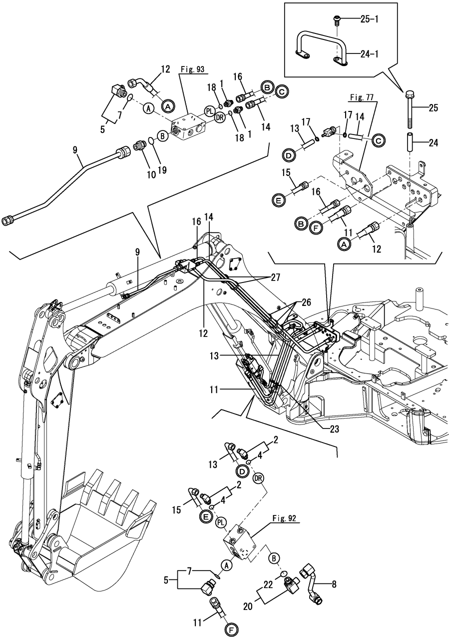
Fig.95. HOLDING VALVE KIT(4)(OPTIONAL)
