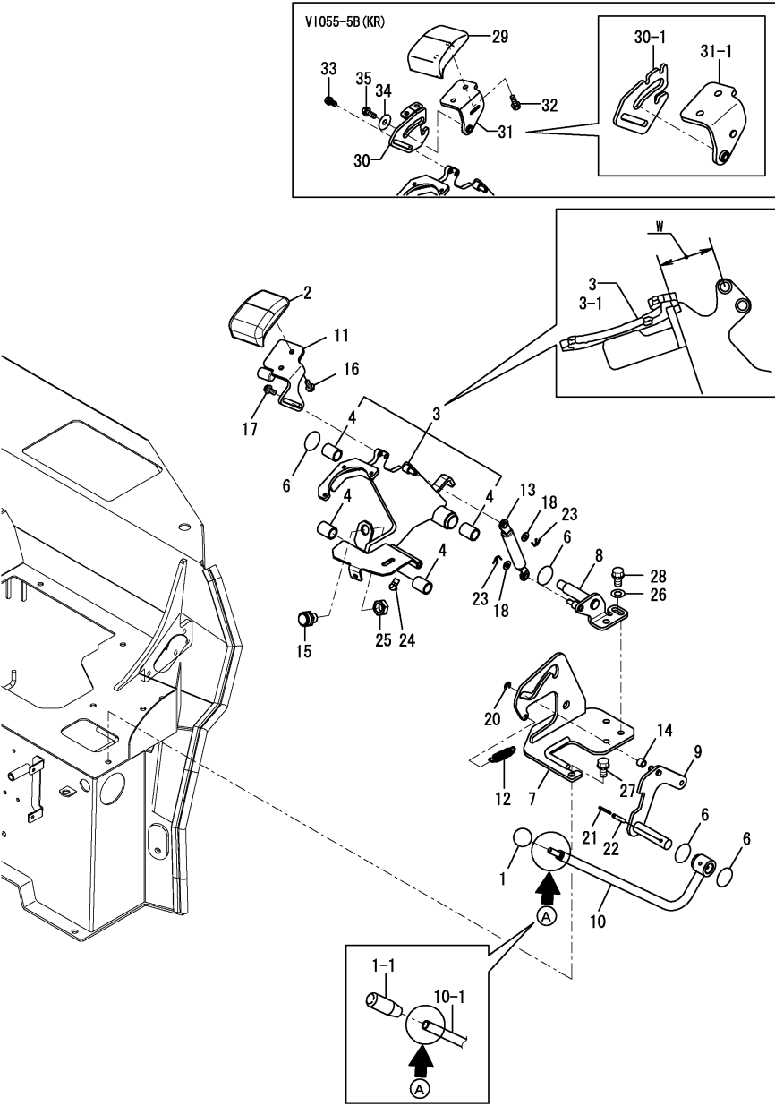
OCS10-M51901 CONTROL EQUIPMENT Fig.24. LOCK LEVER & STAND(LEFT)
