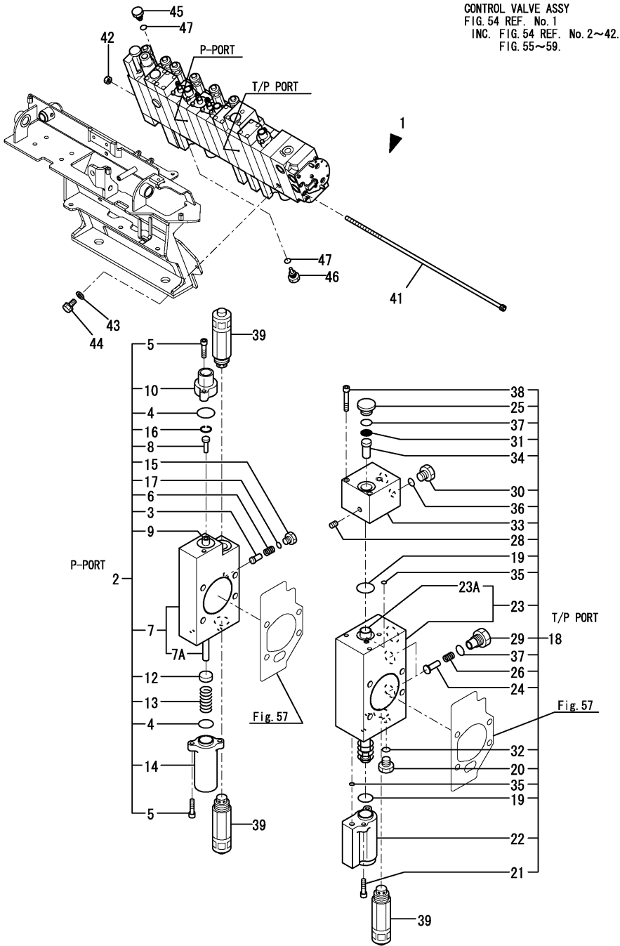
Fig.54. CONTROL VALVE(1/6)(US : TO M54865, AS, NZ, KR)
