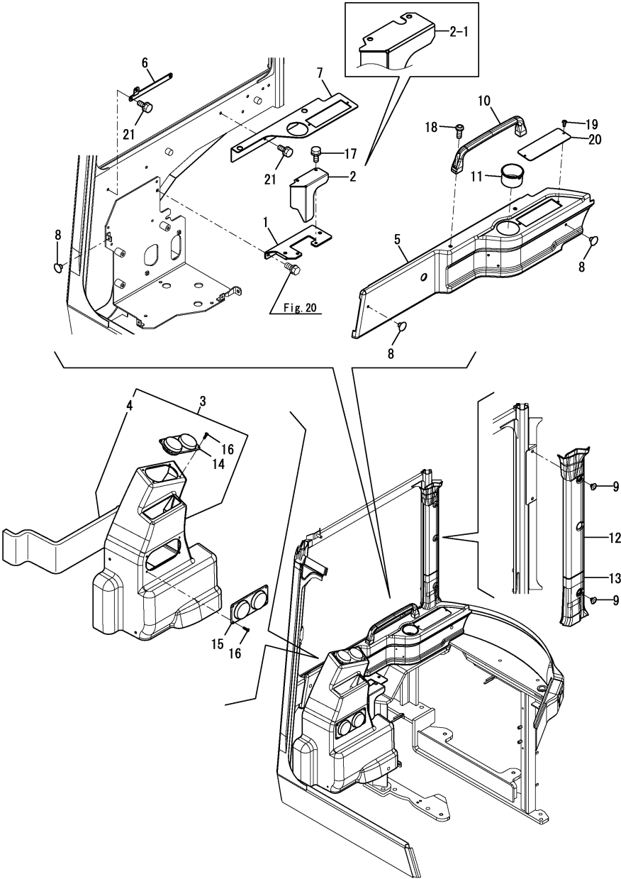
Fig.34. COVER(CABIN)(1)(TO M54180)
