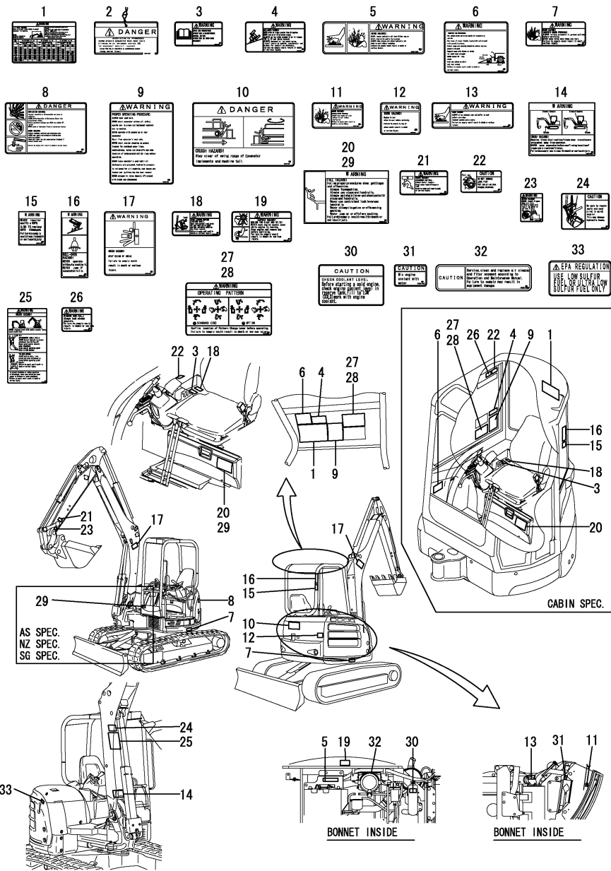
Fig.3. LABEL(SAFETY)
