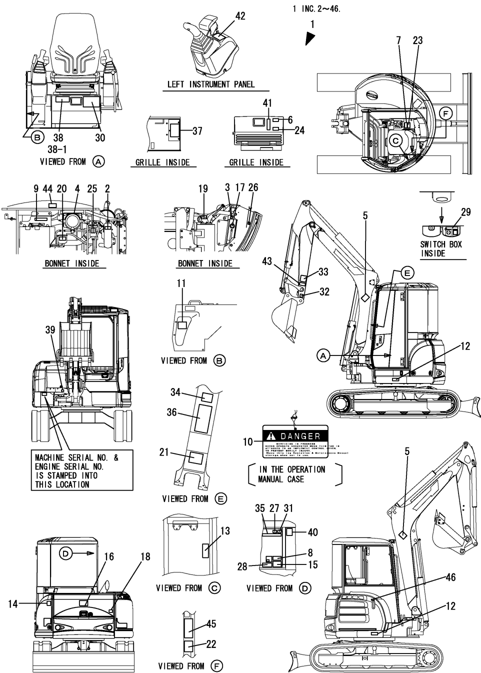
Fig.125. LABEL KIT(FOR CANADA)(OPTIONAL)
