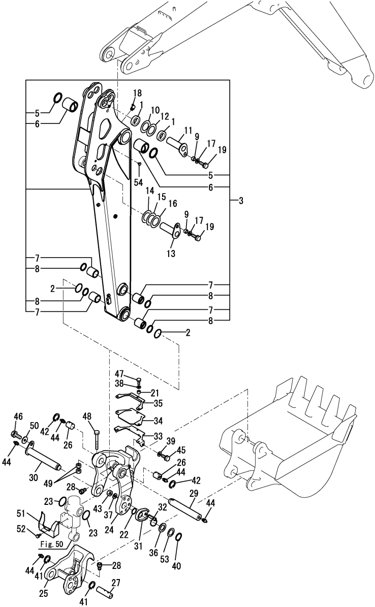
OCS10-M51901 IMPLEMENT Fig.86. ARM & QUICK COUPLER
