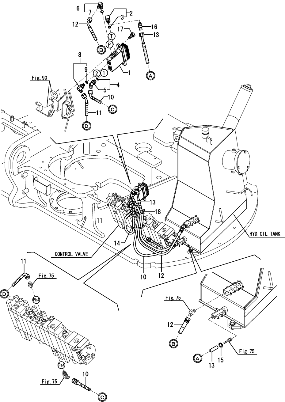
Fig.91. CONTROL PIPING(P.T.O.)
