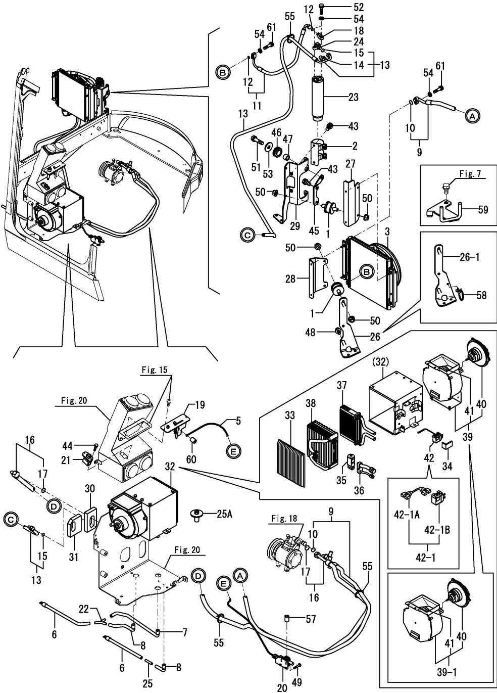
OCS10-M51901 AIR CONDITIONER & HEATER Fig.19. PIPING(AIR CONDITIONER SPEC.)
